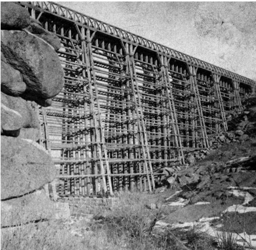
[Originally a stereocard] Plate 112 by Andrew J. Russell showing the Dale Creek Bridge from below, 1868.
